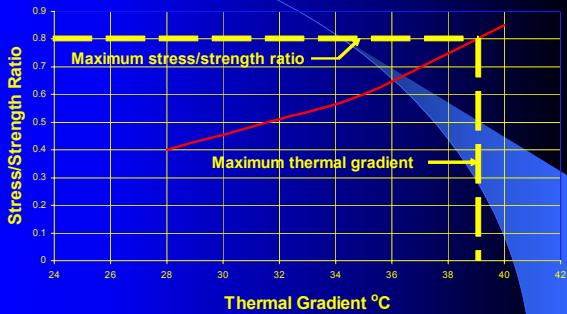
Approximate Stress vs Temperature Gradient
