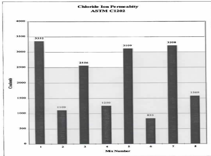
Figure 9: Chloride Ion Permeability
